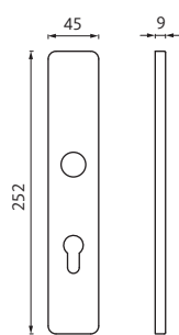
Long backplate, square
