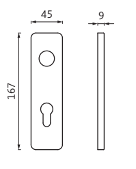
Short backplate, square
