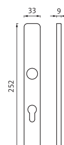
Long backplate, square
