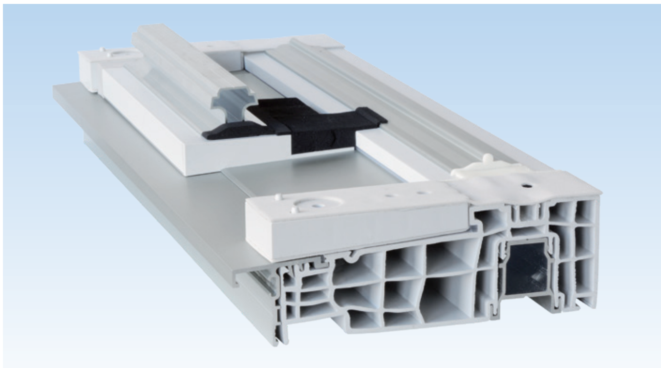
Threshold pre-assembled to the highest degree of fabrication (above: the GU-thermostep 204 for Veka Slide 82)
