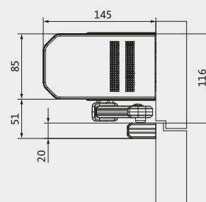
Transom installation Hinge-side – slide rail
